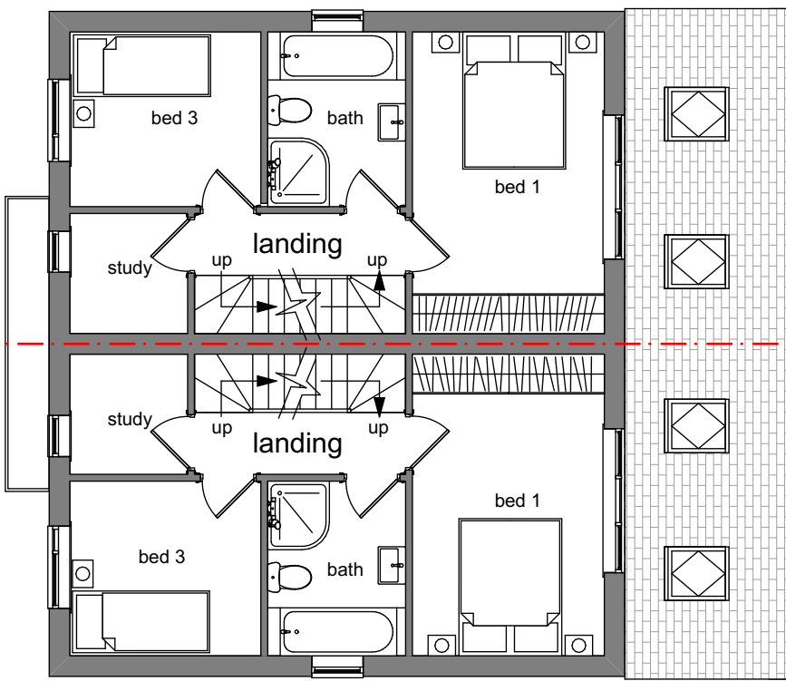
First Floor Plan (units 1 - 6)
