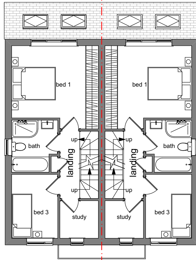
First Floor Plan (units 7 - 12)
