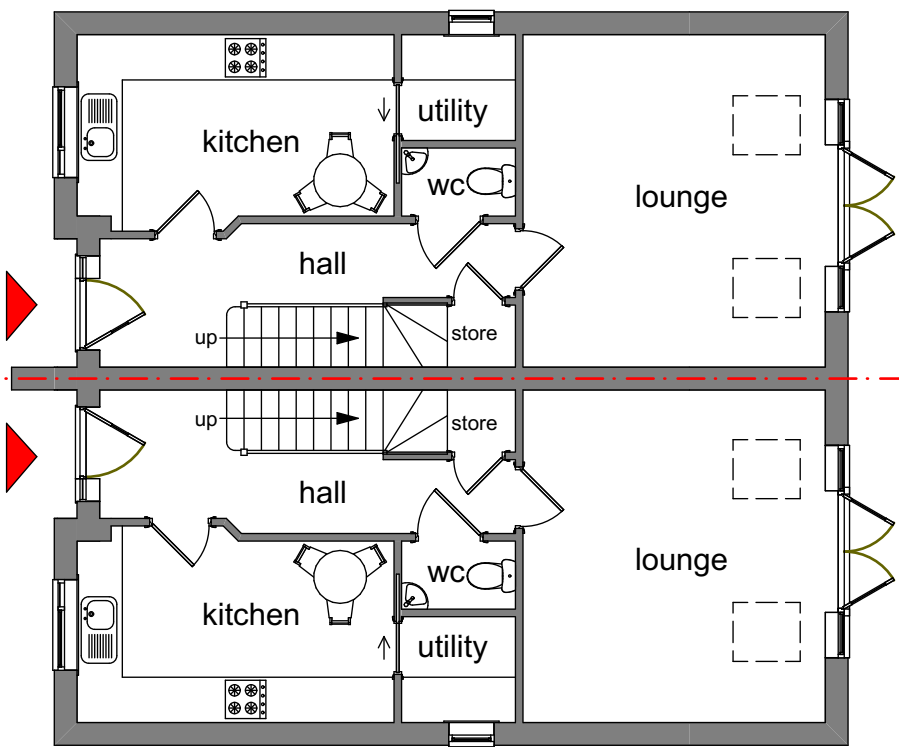
Ground Floor Plan (units 1 - 6) Acre Street
