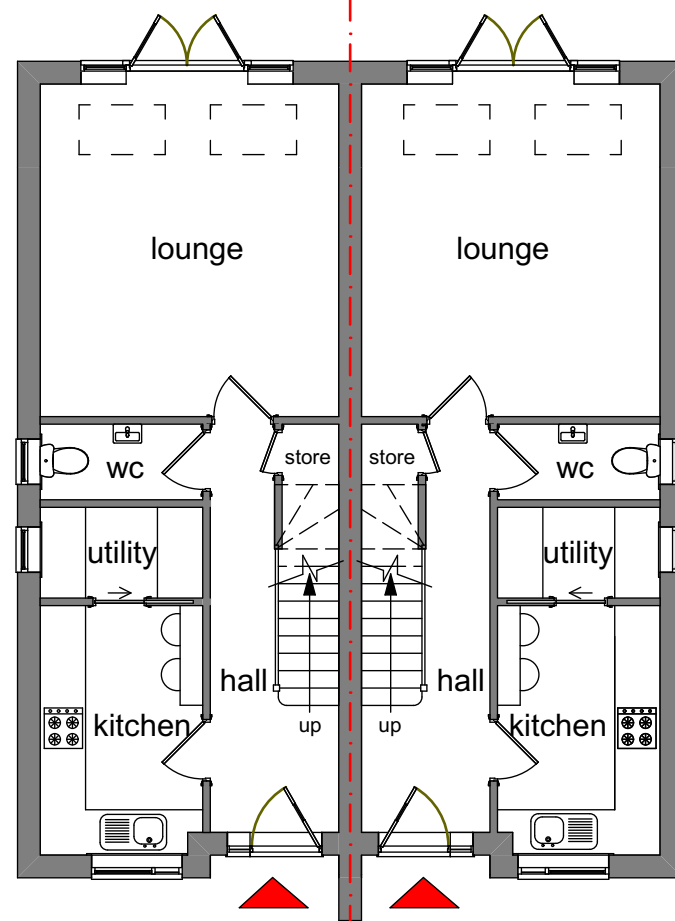
Ground Floor Plan (units 7 - 12) Town Lane
