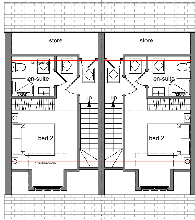
Second Floor Plan (units 7 - 12)
