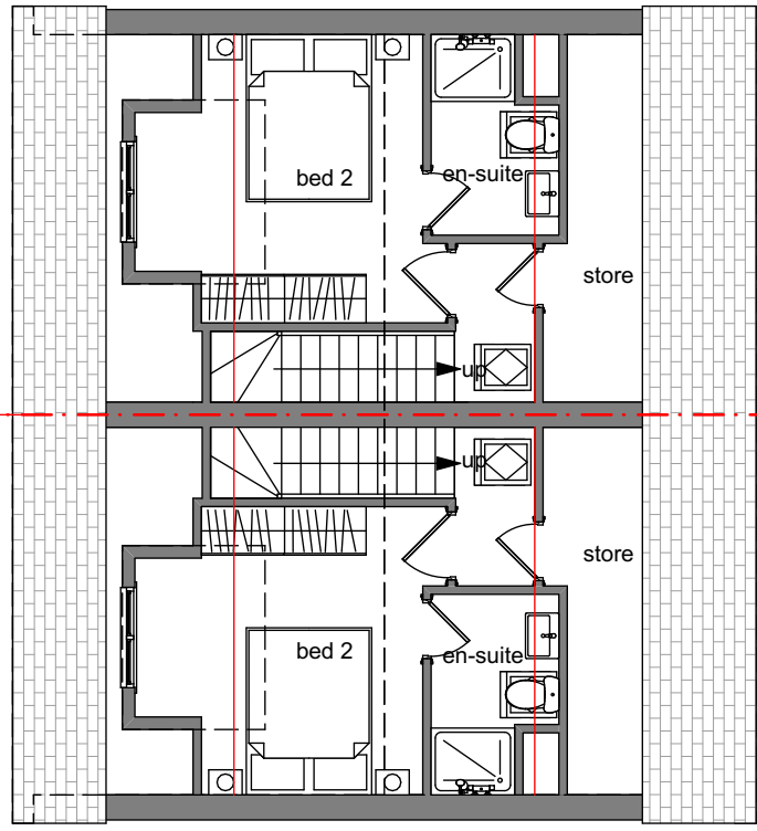
Second Floor Plan (units 1 - 6)
